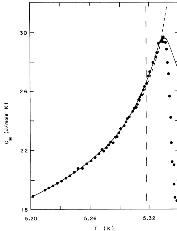
FIG. 4. Comparison of the best fit to the data below T_{\max} using an undamped divergence and using the damped divergence produced when T is treated as complex. For the undamped fit, data falling to the right of the dashed line were discarded as "effected by the rounding." Some data lying at higher temperatures than T_{\max} are also shown to aid in the location of T_{\max} .
